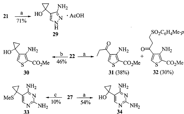
Scheme 9. Deprotection of hetaryl cyclopropyl allyl ethers: a) \text{PdCl}_2 (0.6–0.8 equiv.), AcONa, AcOH, p\text{MeC}_6\text{H}_4\text{SO}_2\text{Li} (1.1–1.5 equiv.), \text{Pd}(\text{Ph}_3\text{P})_4 (7 mol %), 40 °C, 30–90 min; b) \text{Ti}(\text{O}i\text{Pr})_4 (2 equiv.), c\text{HexMgBr} (6 equiv.), \text{Et}_2\text{O} , 20 °C, 16 h; c) t\text{BuOK} (4 equiv.), DMSO, 85–95 °C, 1.5 h
