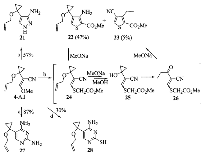
Scheme 8. Condensation reactions of 4-All , affording various O -allyl ethers of 1-heteroaryl cyclopropanols: a) \text{NH}_2\text{NH}_2 , MeOH, reflux, 16 h; b) \text{HSCH}_2\text{CO}_2\text{Me} , MeONa, MeOH, reflux, 16 h; c) guanidine-HCl, MeONa, MeOH, reflux, 24 h; d) thiourea, MeONa, MeOH, reflux, 24 h
