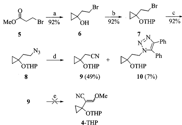
Scheme 3. Attempted synthesis of 4-THP from methyl 3-bromopropionate: a) \text{EtMgBr} (2.2 equiv.), \text{Ti}(\text{OiPr})_4 (0.1 equiv.), \text{Et}_2\text{O}/\text{THF} , 20 °C, 4 h; b) 3,4-dihydro-2H-pyran, \text{py-TsOH} , \text{CH}_2\text{Cl}_2 , 0 \rightarrow 20 °C, 16 h; c) \text{NaN}_3 , DMF, 75 °C, 4 h; d) diphenylacetylene, 10% \text{Pd/C} , p -xylene, reflux, 6 h; e) \text{KH} , \text{HCO}_2\text{Me} , THF, 0 \rightarrow 20 °C; (\text{MeO})_2\text{SO}_2 , 18-crown-6, 20 \rightarrow 50 °C
