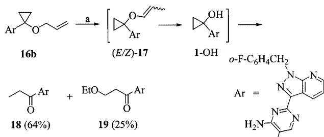
Scheme 6. Opening of the cyclopropanol ring during deprotection of the allyl ether 16b : a) 10% Pd/C, EtOH, 1 M aq. HCl, reflux, 40 h
