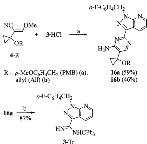
Scheme 5. Synthesis of the O -protected precursors 16a and 16b of the metabolite 1-OH : a) EtOH, EtONa, reflux, 20 h; b) Ph 3 CBF 4 (2 equiv.), CH 2 Cl 2 , room temp., 16 h; reflux, 5 h
