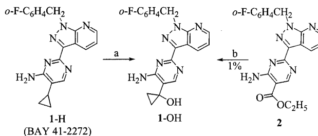
Scheme 1. Isolation of 1-heteroarylcylopropanol 1-OH , a main metabolite of BAY 41-2272 in rats and dogs; [1] reagents and conditions: [3] a) rat hepatocytes (in vivo); b) Sm/CH 2 I 2 , THF, 50 °C, 70 min; 1 M HCl; RP18 chromatography, 1%
