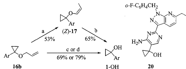
Scheme 7. Synthesis of the metabolite 1-OH by deprotection of the allyl ether 16b : a) t BuOK (2 equiv.), DMSO, 85–95 °C, 1.5 h; b) 0.5 M aq. HCl, MeOH, 55–60 °C, 1.5 h; c) THF/diethyl ether, c HexMgBr (1 equiv.), Ti(O i Pr) 4 (1 equiv.), then c HexMgBr (4 equiv.), 10 → 20 °C, 3 h; d) PdCl 2 (1 equiv.), AcONa, AcOH, p -MeC 6 H 4 SO 2 Li (2.6 equiv.), Pd(Ph 3 P) 4 (13 mol %), 50 °C, 90 min
