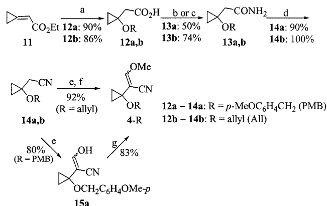
Scheme 4. Synthesis of the main building blocks 4-R : a) \text{ROH} , \text{NaH} , 20 °C, 4 h; b) \text{SOCl}_2 , \text{CH}_2\text{Cl}_2 , reflux, 2 h; \text{concd. aq. NH}_3 ( 13a ); c) N,N' -carbonyldiimidazole, THF, 25 °C, 2.5 h; \text{NH}_4\text{OAc} , 20 °C, 16 h ( 13b ); d) \text{TFAA/py} , \text{CH}_2\text{Cl}_2 , 0 \rightarrow 20 °C, 16 h; e) \text{KH} , \text{HCO}_2\text{Me} , THF, 0 \rightarrow 20 °C, 3 h; f) (\text{MeO})_2\text{SO}_2 , 18-crown-6, 0 \rightarrow 50 °C; g) \text{NaH} , THF, room temp., 2 h, then (\text{MeO})_2\text{SO}_2 , 40 °C, 2 h
