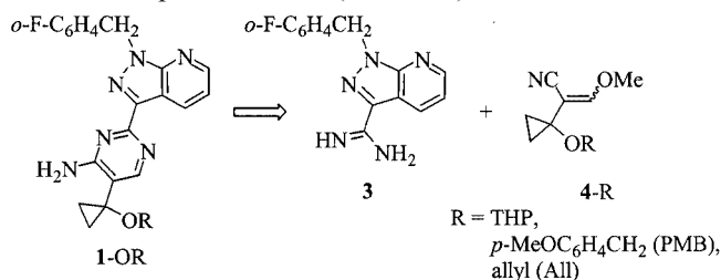
Scheme 2. Synthetic strategy for the construction of 1-heterylcyclopropanol 1-OH
